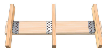
Ledger plate to stud support
