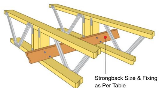
PRYDA SPAN STRONGBACK
