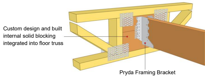
Pryda Framing Bracket
