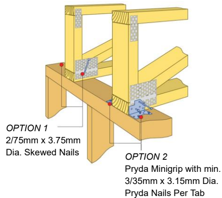
TYPICAL PLATE SUPPORT FIXING
