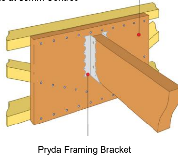
Pryda Framing Bracket
