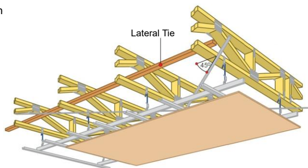
Dynamics of different beam types, floor truss spans and loading conditions shall be assessed simultaneously as a system.
