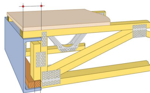
Min. Bearing 30mm on Primary Bearing Point
