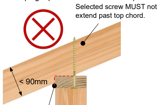
Figure 5 - Sloping top chord / rafter with roof pitch between 22.5° – 35° degrees on 90 x 35mm top plate.
