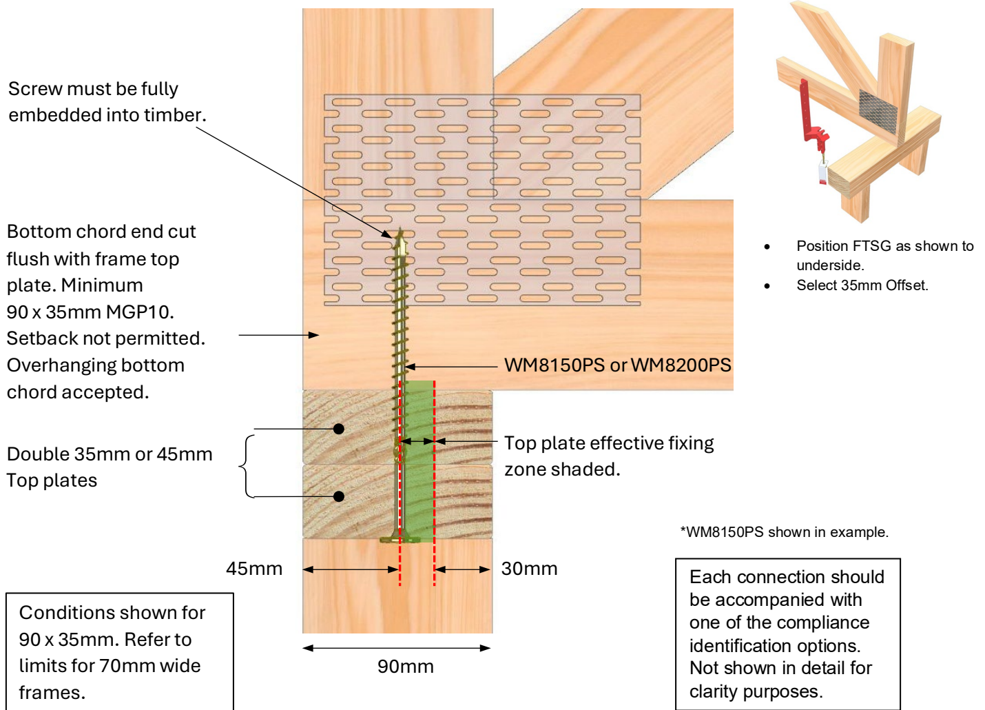
Figure 6 – illustration showing effective fixing zone for support condition with truss bottom chord end cut flush with supporting wall double top plates.
