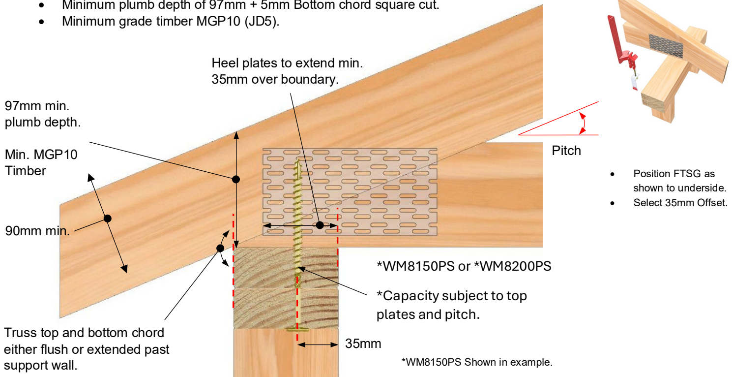
Figure 8 – Truss heel on double top plates.
