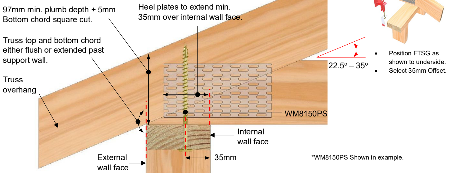
Figure 4 – Truss heel with roof pitch between 22.5 – 35 degrees on 90 x 35mm top plate.
