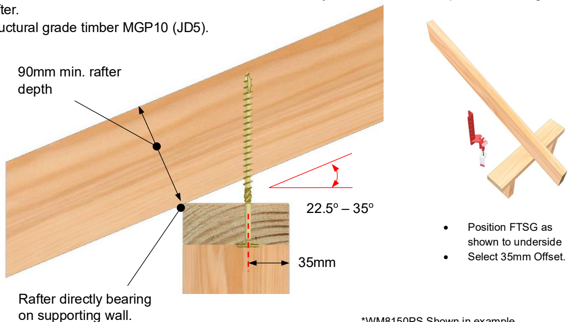
Figure 5 - Sloping top chord / rafter with roof pitch between 22.5° – 35° degrees on 90 x 35mm top plate.
