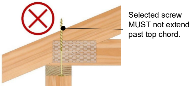
Figure 4 – Truss heel with roof pitch between 22.5 – 35 degrees on 90 x 35mm top plate.
