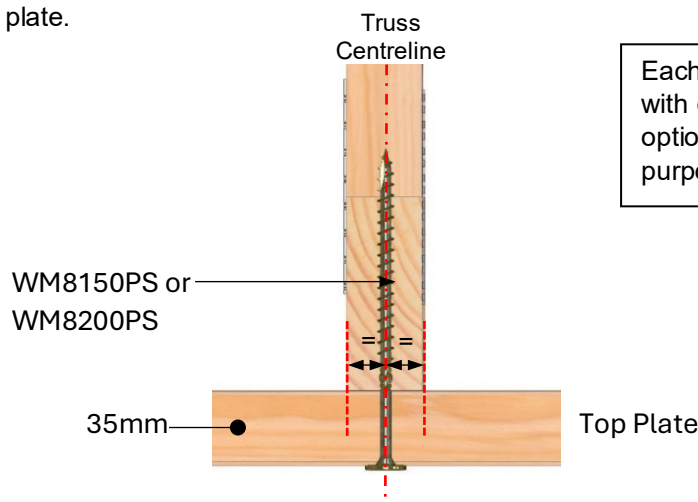
Figure 2 – illustration showing screw installed centreline of truss bottom.
