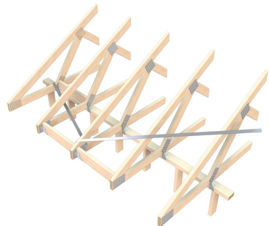
FIXING DETAILS FOR CANTILEVERS
