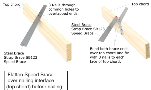
(a) Lap Splice
