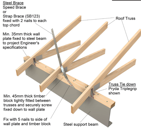
END FIXING DETAILS FOR STEEL BEAM
