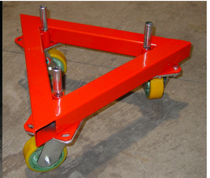
Triangular truss trolley
