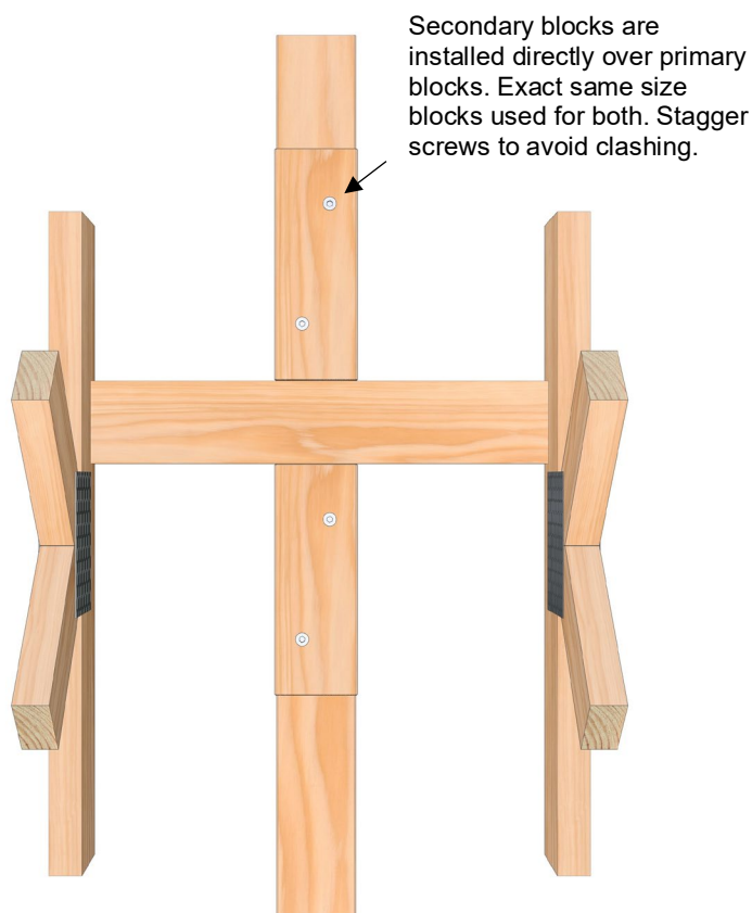
Secondary blocks installation.
