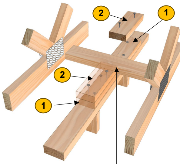
Shear block overlapping trimmer
