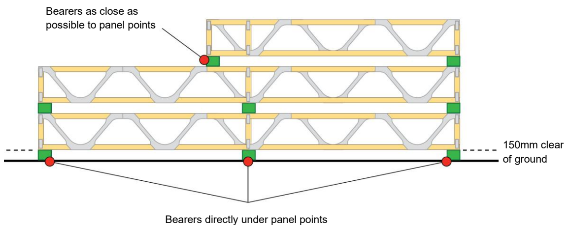
Figure 4: Storage - Floor trusses stacked vertically
