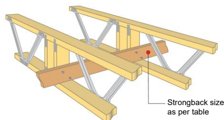
Figure 41: Pryda Span Strongback.
