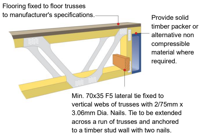
Figure 11: Alternative fixing to steel beam.
