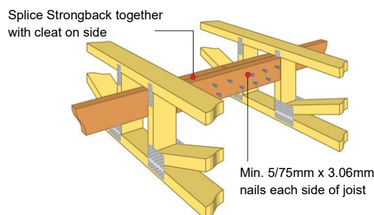
Figure 43: Alternative Strongback splice.
