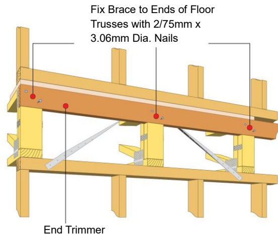
Figure 6b: Brace not wrapped under the wall plate is not recommended.
