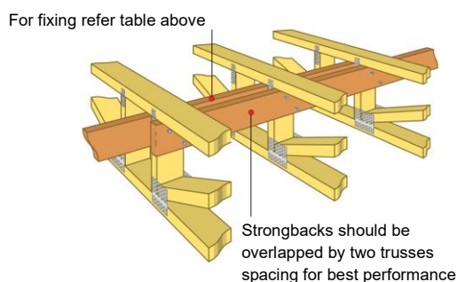
Figure 42: Strongback splice.
