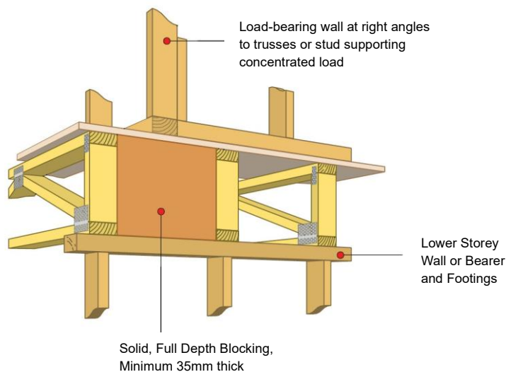
Figure 30: Blocking under wall or concentrated loads.
