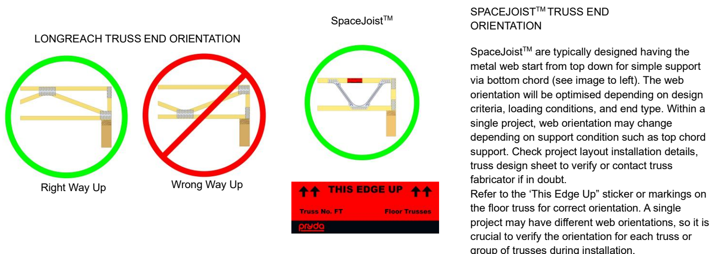
Figure 1: Pryda Floor Truss Orientation.
