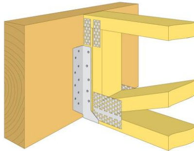
Figure 14: Typical face fixed connection using framing brackets.
