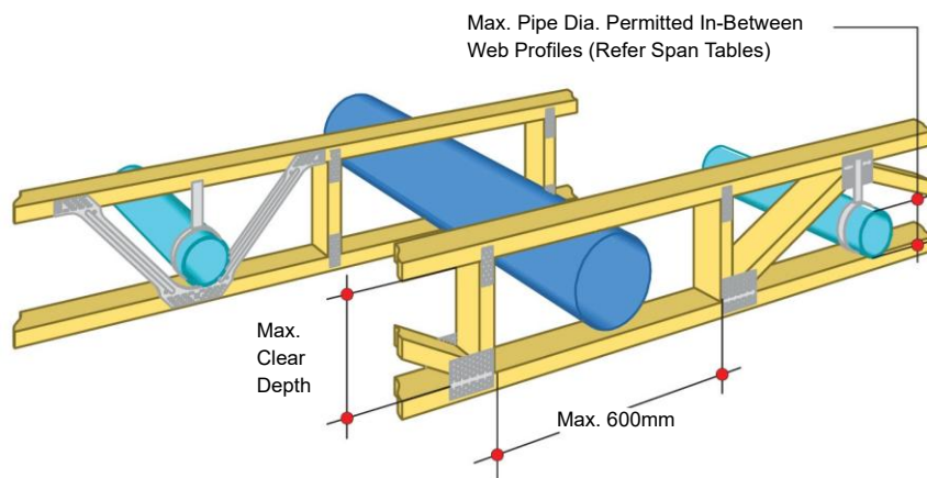
Figure 32: Centre gap for mechanical services
