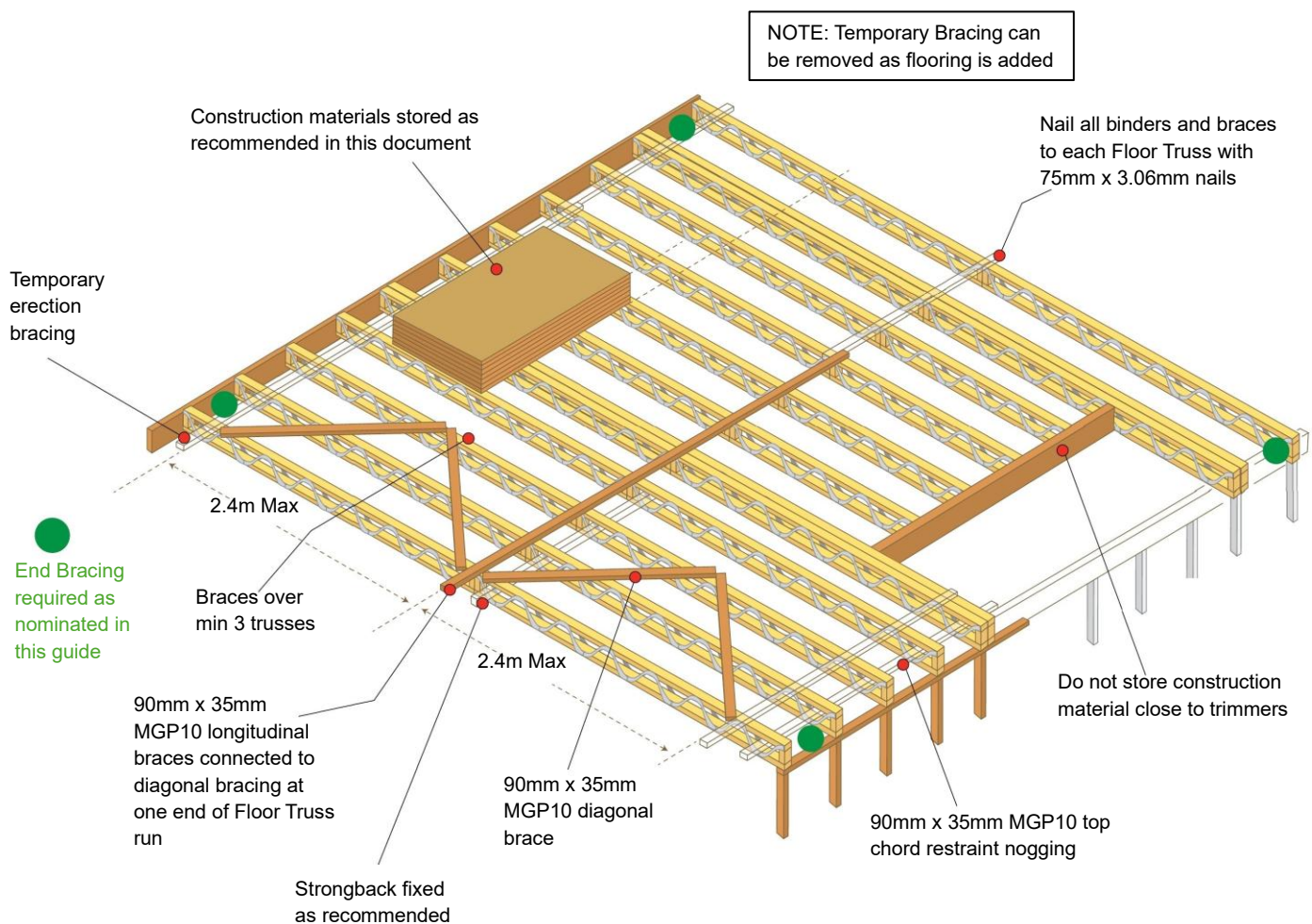
Figure 5: Bracing
