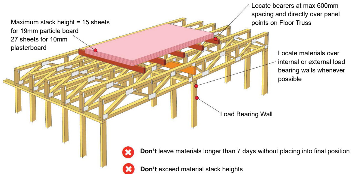
Figure 21: Stacking of material parallel to trusses.
