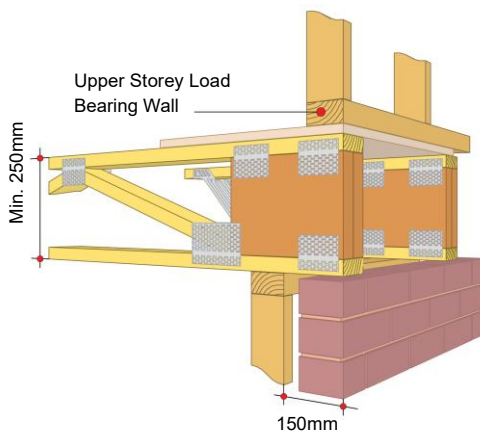
Figure 36: Cantilever - Perpendicular off-set upper load bearing wall.
