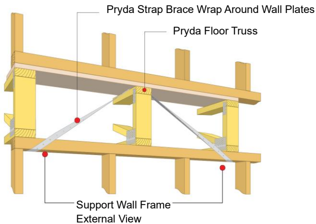
Figure 6a: Brace wrapped under wall plate is the preferred option.
