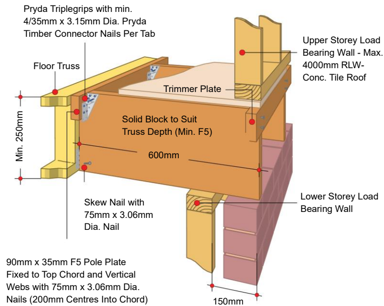
Figure 38: Cantilever - Parallel off-set upper load bearing wall.
