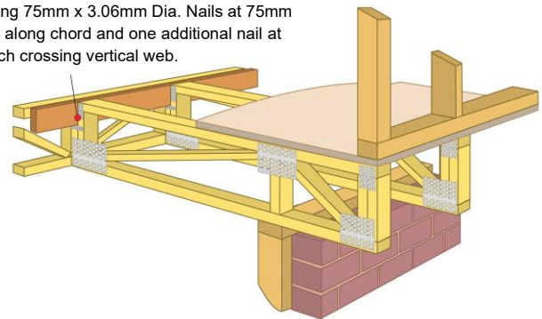
Figure 37: Large Cantilever - Parallel off-set upper load bearing wall.
