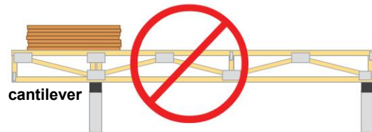
Figure 19: Never stack materials on the cantilever of a truss.
