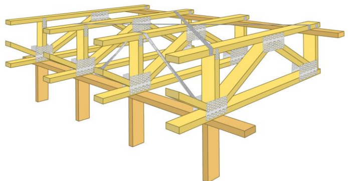
Figure 8: Bracing walls supported by cantilever.
