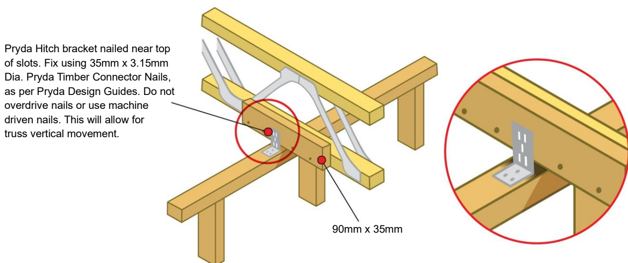
Figure 28: Truss perpendicular to non-bracing wall.
