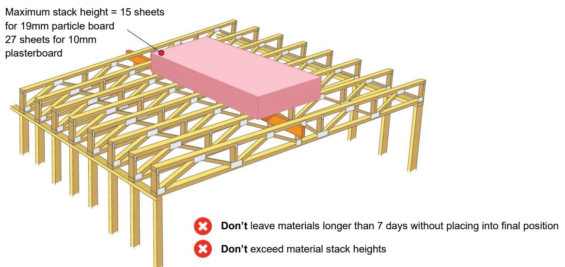
Figure 22: Stacking of materials perpendicular to trusses.
