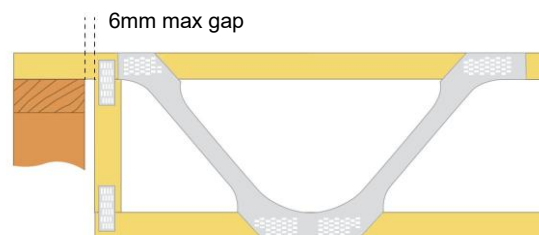
Figure 13: Typical top chord support fixing.
