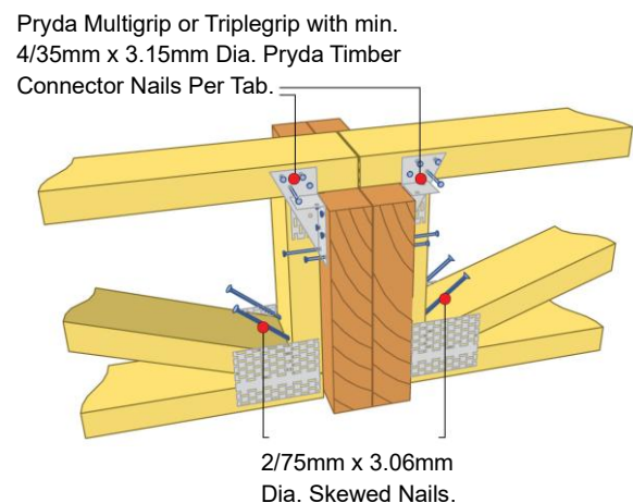
Figure 12: Typical fixing to timber beam.
