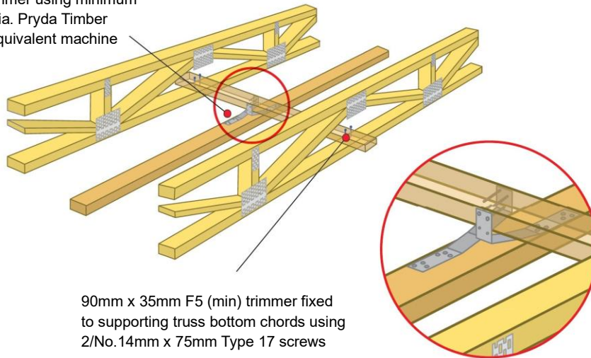
Figure 25: Walls parallel.
