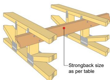
Figure 40: Longreach Strongback.
