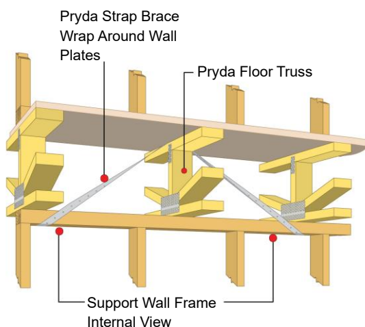
Figure 7: Internal bracing for stability and wind.
