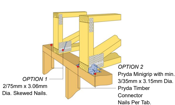
Figure 9: Typical plate support fixing.
