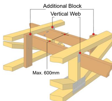
Fig 44 - Non-Aligned Strongbacks.
