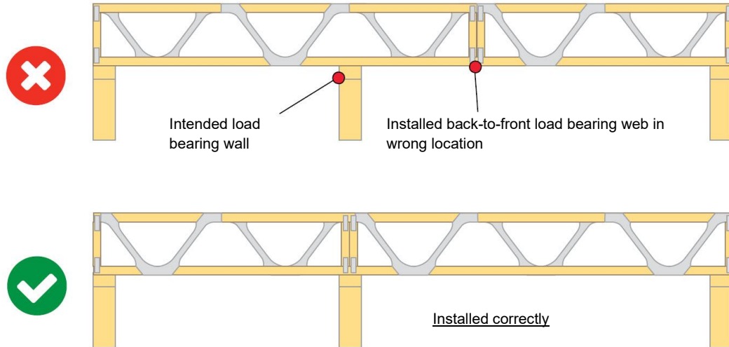
Figure 23: Common installation errors.
