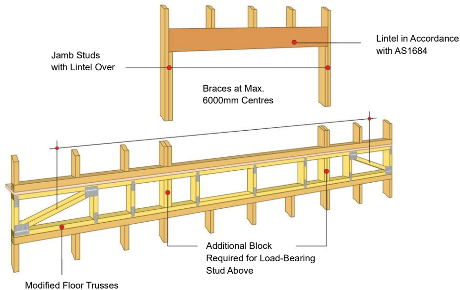
Figure 29: Fully supported end truss.
