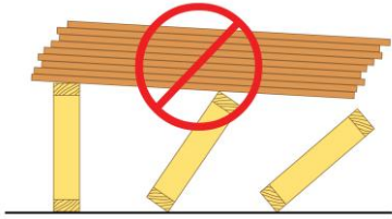
Figure 16: Don't stack materials on unbraced trusses.
