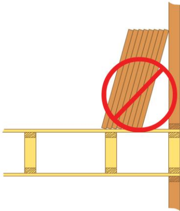
Figure 17: Don't allow the stack to lean against walls. Don't stack materials in concentrated areas so that they overload a single or small group of trusses.
