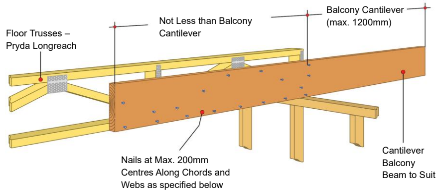
Figure 35: Cantilevered solid joist detail.
