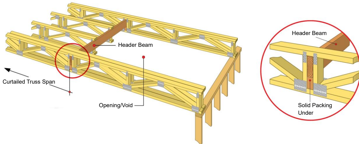
Figure 31: Floor openings.
