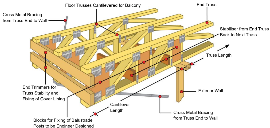
Figure 34: Cantilevered truss end detail.
