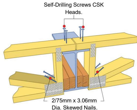
Figure 10: Typical fixing to steel beam.
