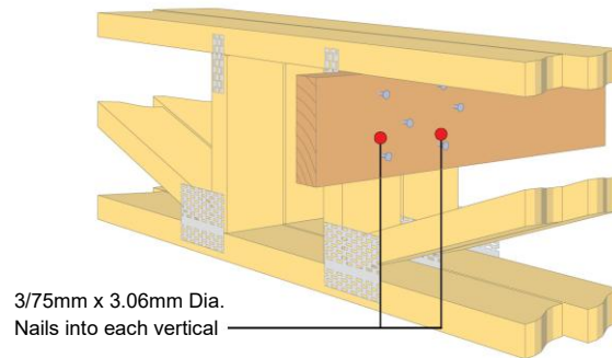
Figure 33: Multiple truss fixing.
