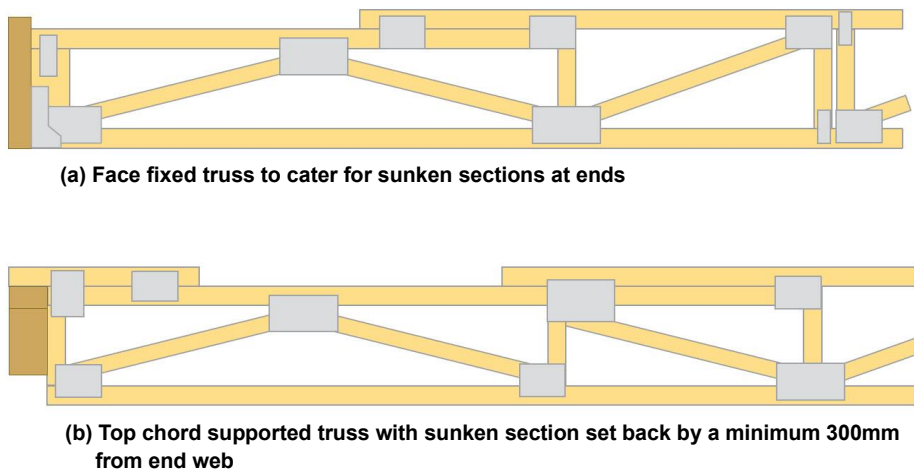
Figure 24: Sunken Sections support types.
