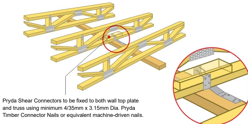
Figure 26: Walls perpendicular.
