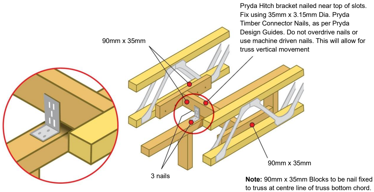
Figure 27: Truss parallel to non-bracing wall.
