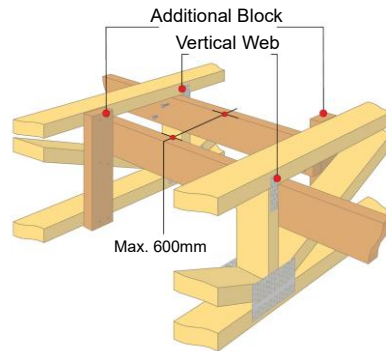
Fig 44 - Non-Aligned Strongbacks.
