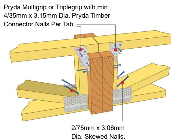
Figure 12: Typical fixing to timber beam.
