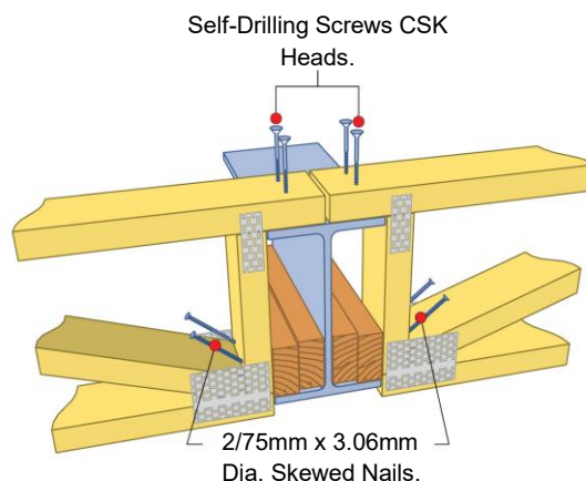
Figure 10: Typical fixing to steel beam.
