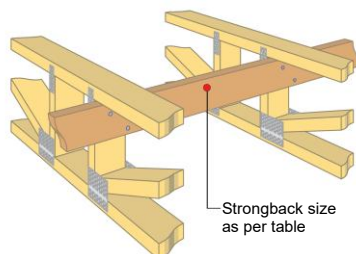
Figure 40: Longreach Strongback.
