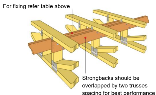
Figure 42: Strongback splice.
