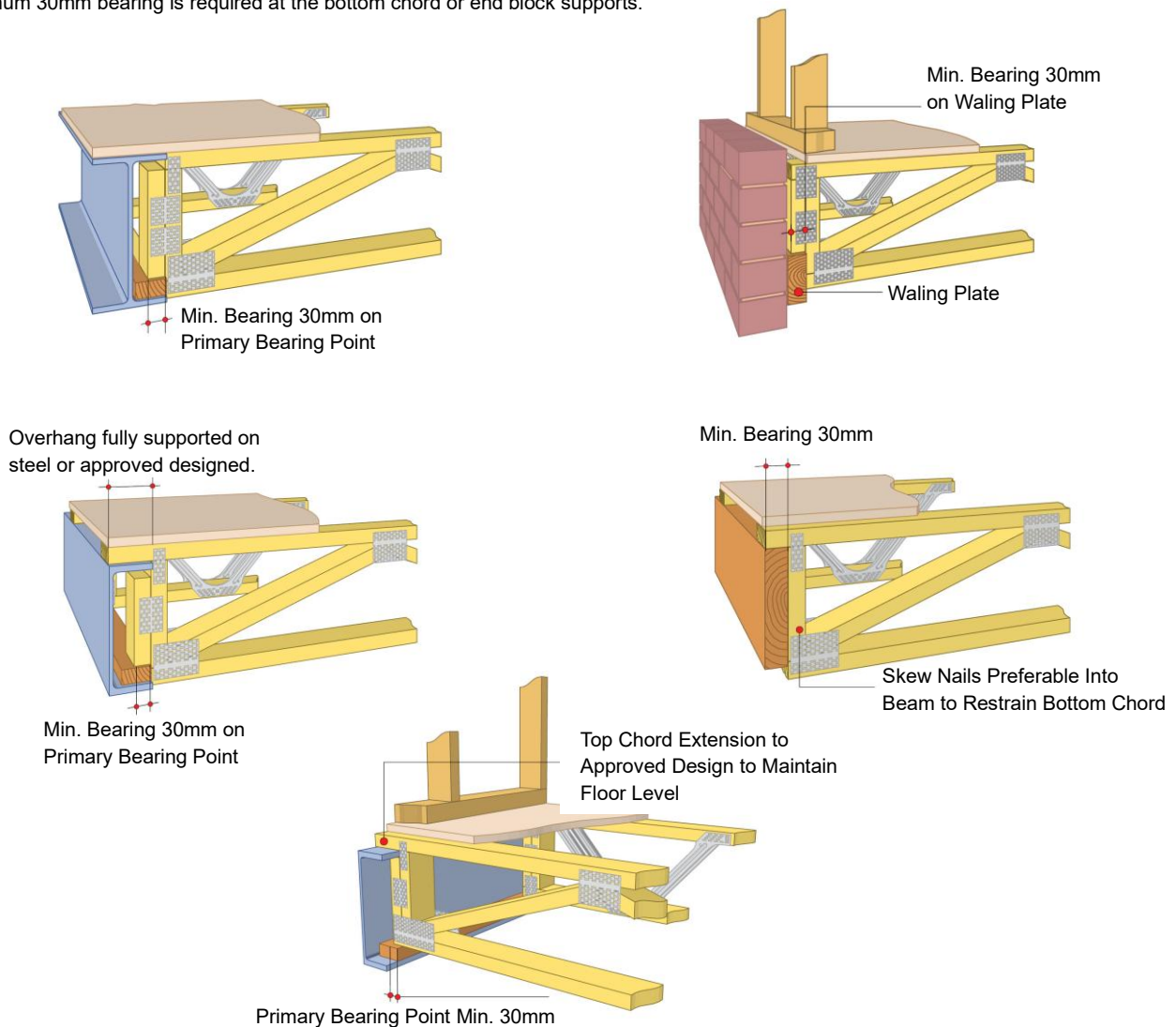
Figure 15: Bottom chord or end block supports bearing.
