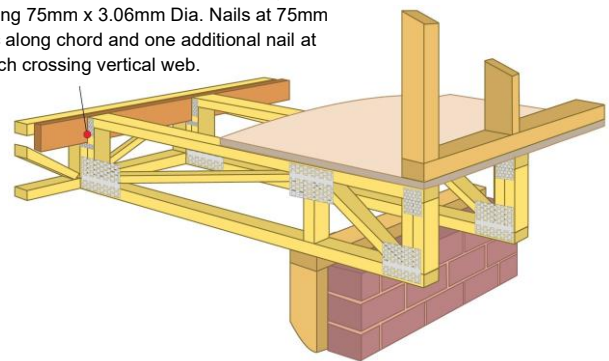
Figure 37: Large Cantilever - Parallel off-set upper load bearing wall.
