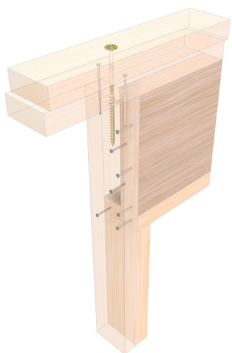
Top plates to jamb stud connections
