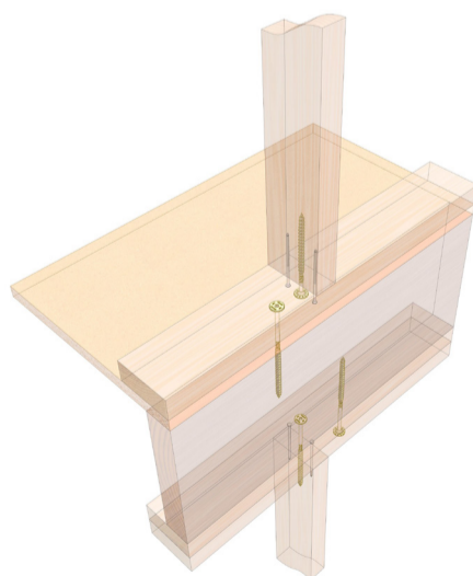
Single plate to beam connections
