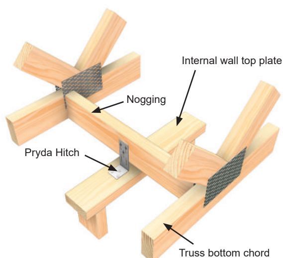
Wall Parallel to Trusses
